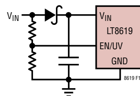
Figure 10. Reverse V_{IN} Protection
