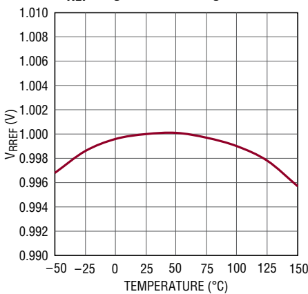
R_{\text{REF}} Regulation Voltage
