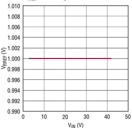
R_{\text{REF}} Line Regulation
