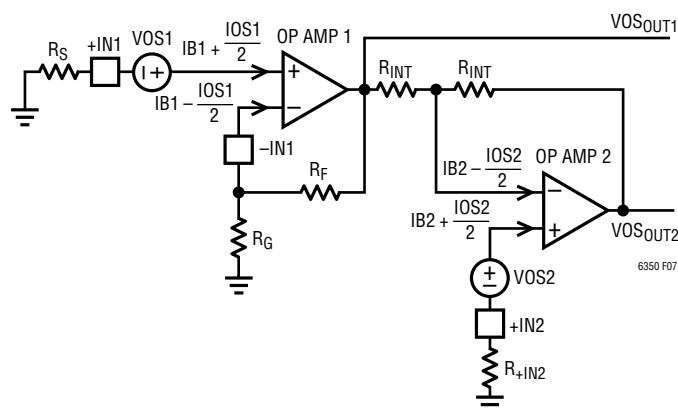
Figure 7. Offset Model
