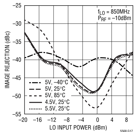
Figure 17. Image Rejection vs LO Power
