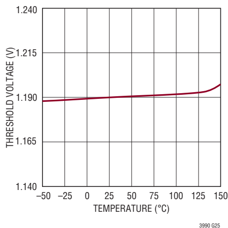
EN/UVLO Threshold
