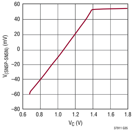
V_{(SNSP-SNSN)} Boost Threshold vs V_C
