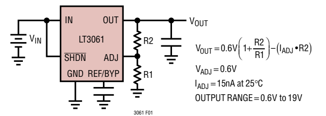
Figure 1. Adjustable Operation
