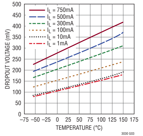
OUT1 Dropout Voltage vs Temperature
