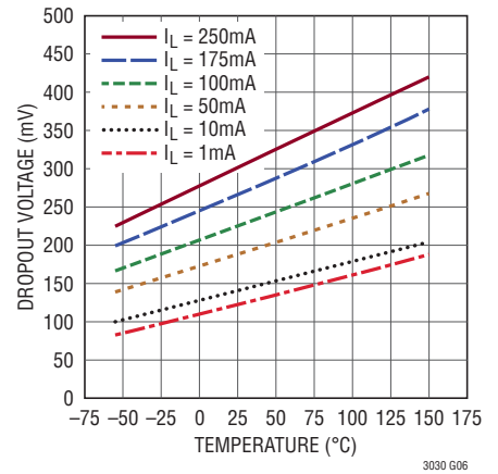
OUT2 Dropout Voltage vs Temperature
