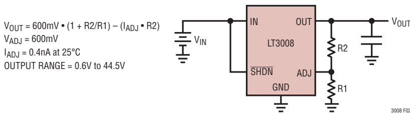
Figure 2. Adjustable Operation
