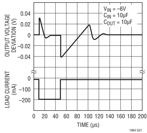
LT1964-5, Transient Response, C_{BYP} = 0.01\mu F
