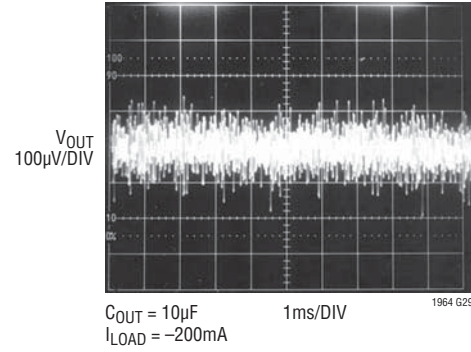
LT1964-5, 10Hz to 100kHz Output Noise, C_{BYP} = 0.01\mu F
