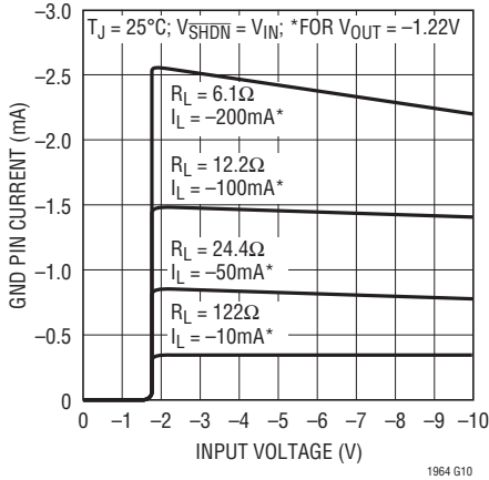
LT1964 GND Pin Current
