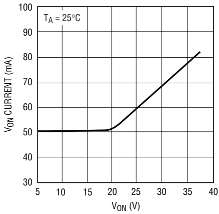
V ON Current Limit
