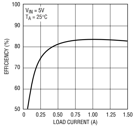
Efficiency, V LOGIC = 3.3V
