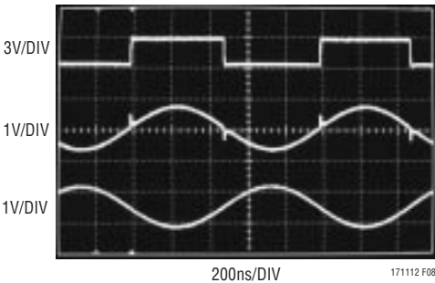
Figure 8. Oscillator Waveforms with V S = 3V. Top is Comparator Output. Middle is Xtal Feedback to Pin 2 at LT1711 (Note the Glitches). Bottom is Buffered, Inverted and Bandpass Filtered with a Q = 5 by LT1806
