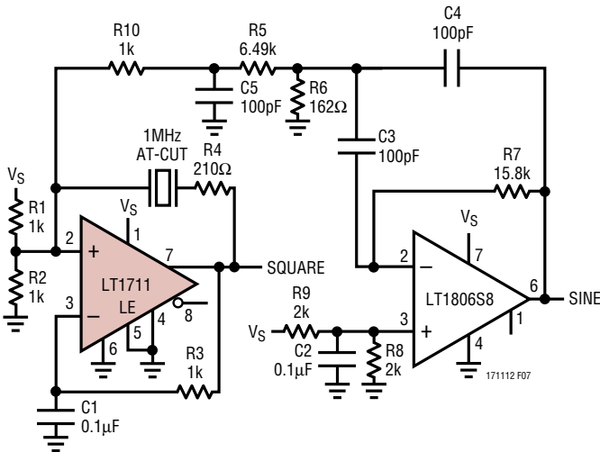
Figure 7. LT1711 Comparator is Configured as a Series Resonant Xtal Oscillator. LT1806 Op Amp is Configured in a Q = 5 Bandpass with f c = 1MHz
