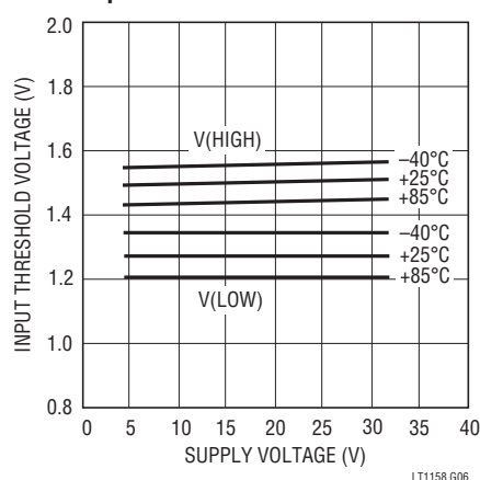
Input Thresholds
