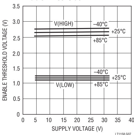
Enable Thresholds
