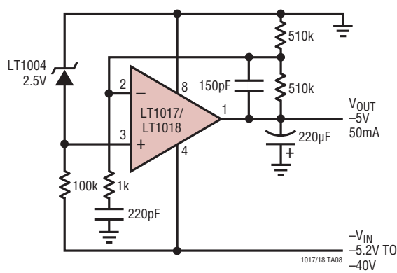
Negative Voltage Regulator
