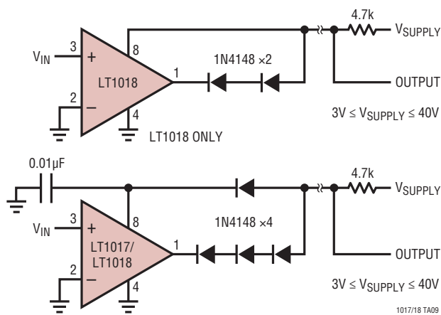
2-Wire Comparator
