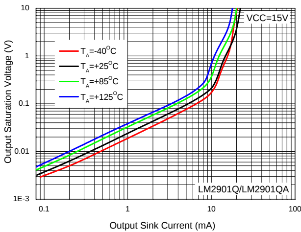
Output Saturation Voltage vs. Sink Current
