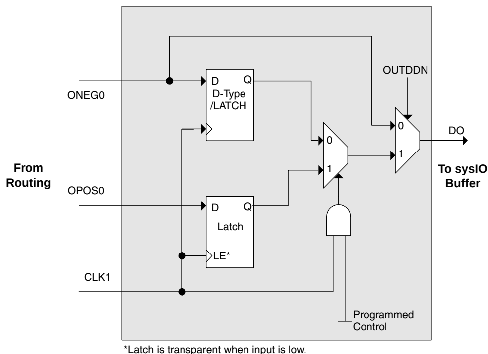
Figure 2-30. ODDRXB Primitive
