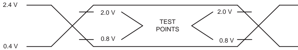
Figure 12. Switching Characteristics
