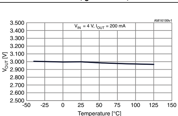
Figure 9. Output voltage vs. temp. for fixed version ( I_O = 200\ \text{mA} )
