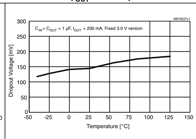
Figure 35. Dropout voltage vs. temperature ( I_{OUT} = 200\text{ mA} )
