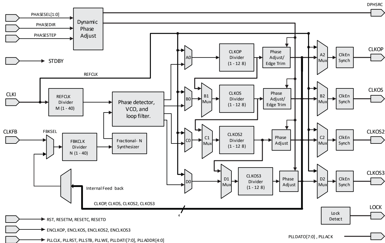
Figure 2.7. PLL Diagram
