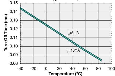
Turn-Off Time vs. Temperature ( I_L=100\text{mA} )
