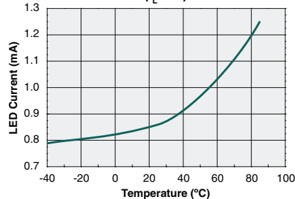
LED Current to Operate vs. Temperature ( I_L=1\text{A} )
