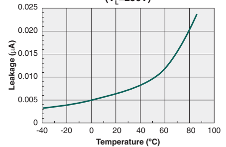
Typical Leakage vs. Temperature Measured across Pins 5&6 or 7&8 ( V_L=250\text{V} )
