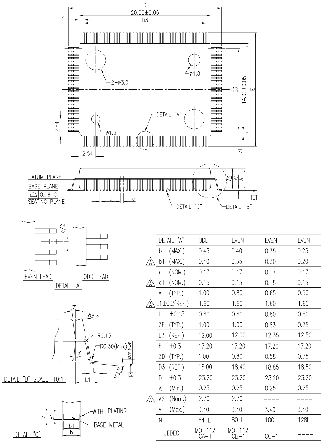
128-Pin PQFP (PQ)
