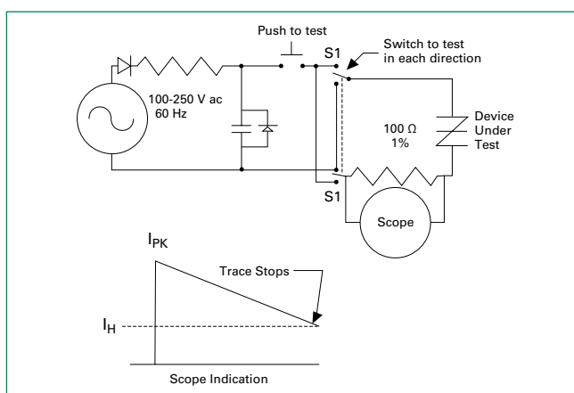
Figure 11: Dynamic Holding Current Test Circuit for SIDACs
