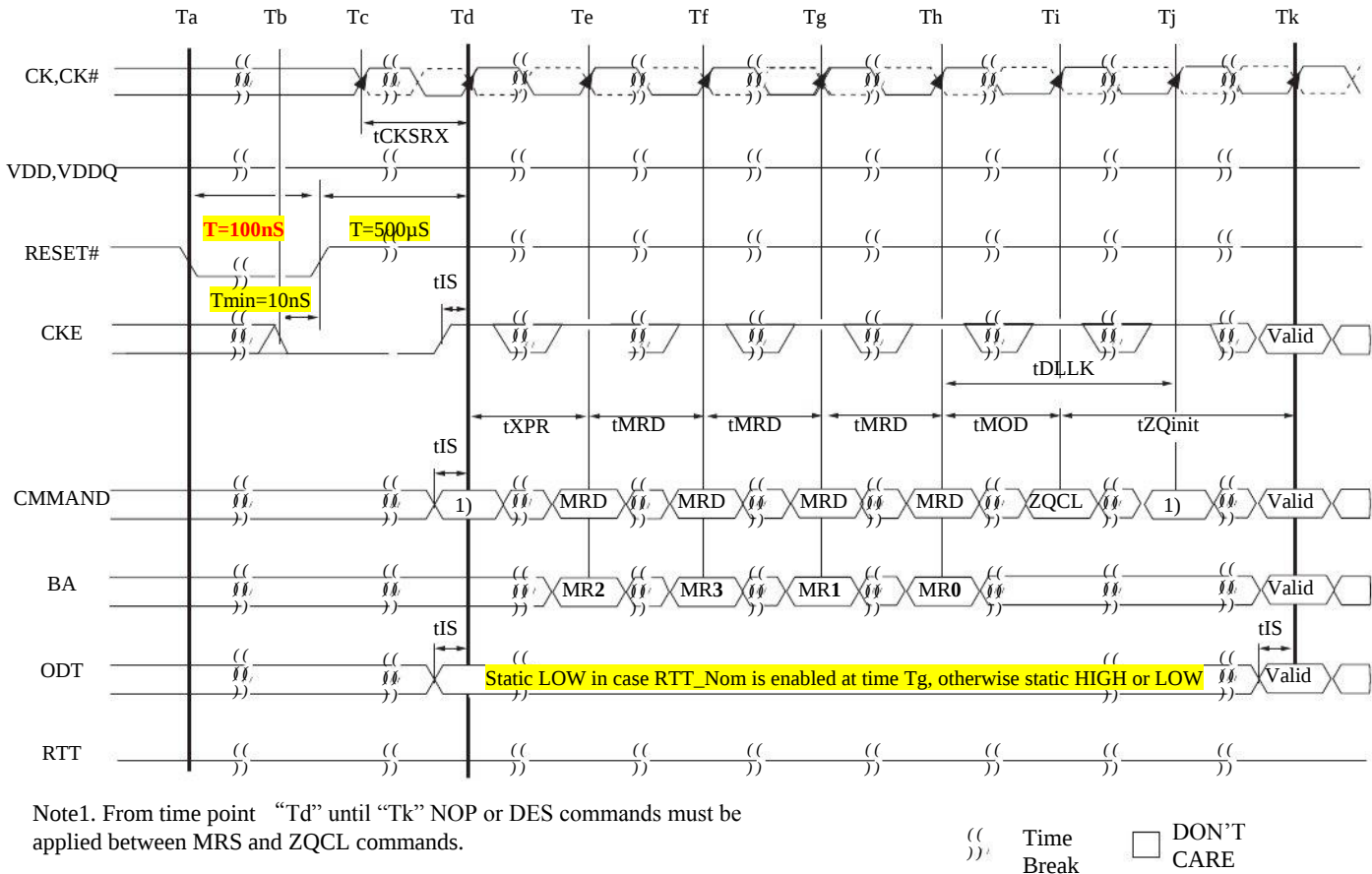
Figure2.1.2 Reset Procedure at Power Stable Condition
