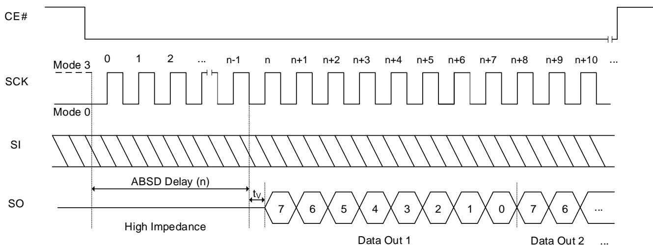
Figure 8.72 AutoBoot Sequence (QE = 0)
