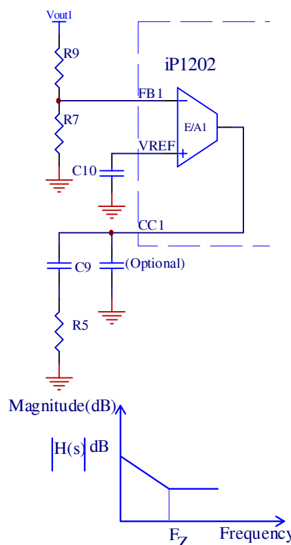
Fig. 18: Typical Type II compensation and its gain plot
