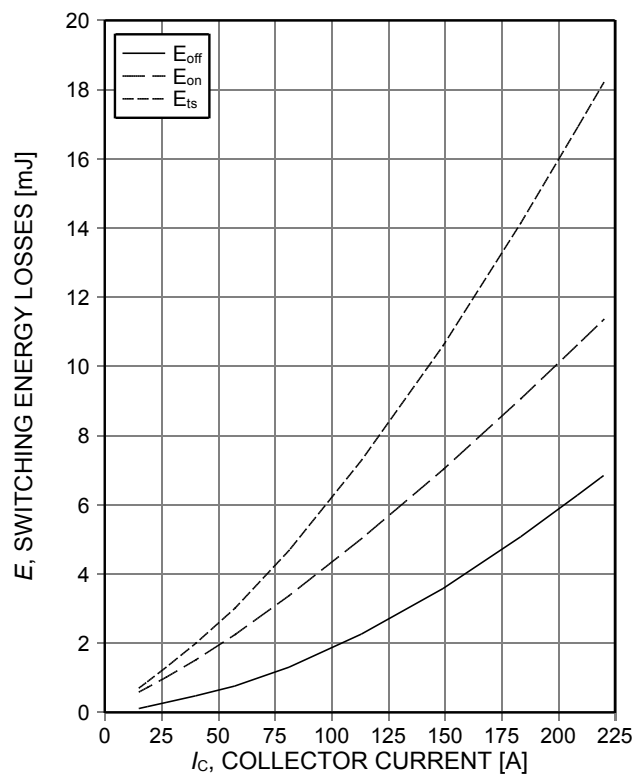
Figure 12. Typical switching energy losses as a function of collector current (inductive load, T_{vj}=150^\circ\text{C} , V_{CE}=400\text{V} , V_{GE}=0/15\text{V} , R_{G(on)}=8\Omega , R_{G(off)}=8\Omega , dynamic test circuit in Figure E)
