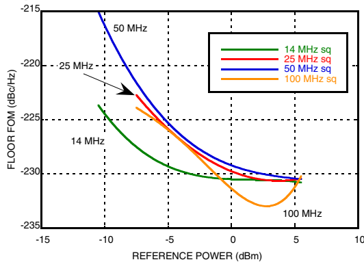
Figure 21. Reference Input Sensitivity, Square Wave, 50 \Omega [9]
