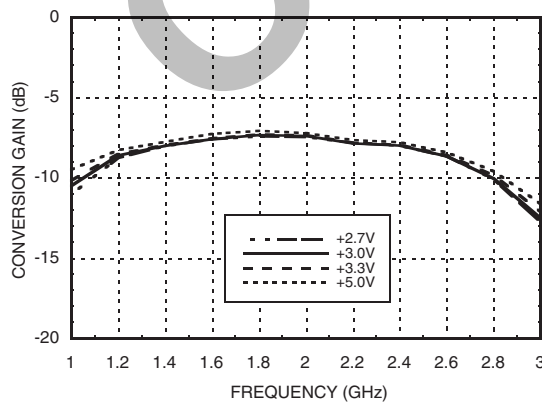
Conversion Gain vs. Vdd @ LO = 0 dBm
