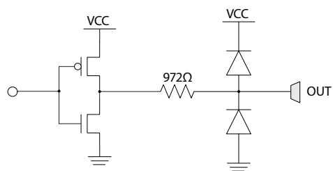
Figure 3-3: Low-speed Outputs (LOCKED, LOS, \text{SD}/\overline{\text{HD}} )
