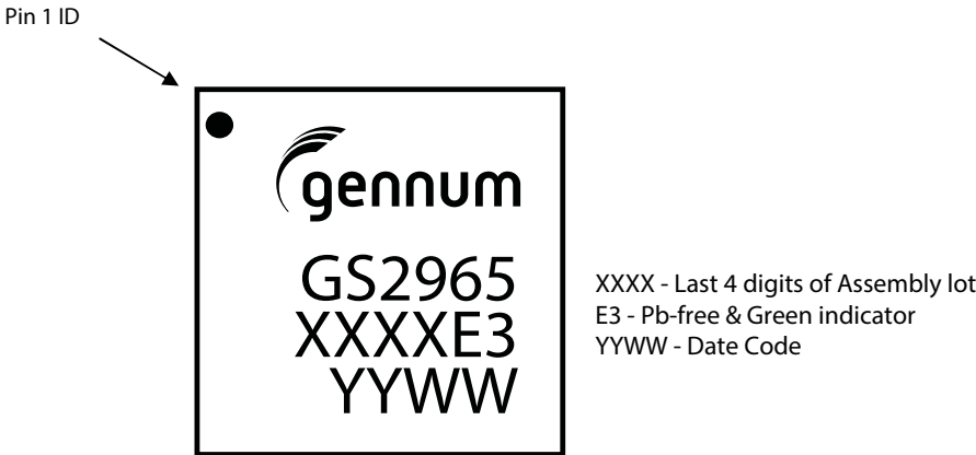
Figure 6-3: Marking Diagram
