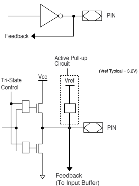
Typical Output
