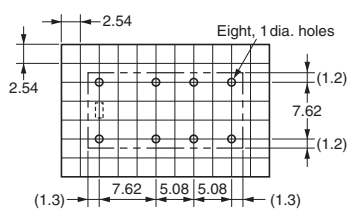
PCB Mounting Holes (Bottom View) Tolerance: ±0.1 mm
