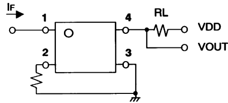
G3VM-61A1
