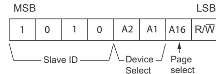
Figure 6. Memory Slave Device Address
