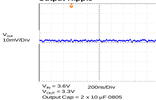
Output Ripple
