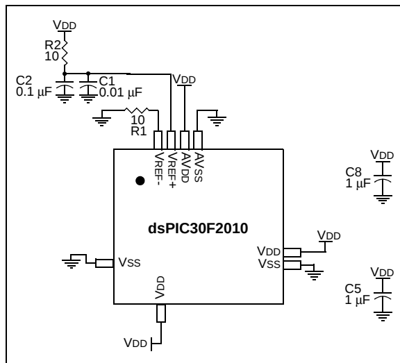
FIGURE 18-2: ADC VOLTAGE REFERENCE SCHEMATIC
