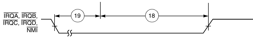
a) First Interrupt Instruction Execution
