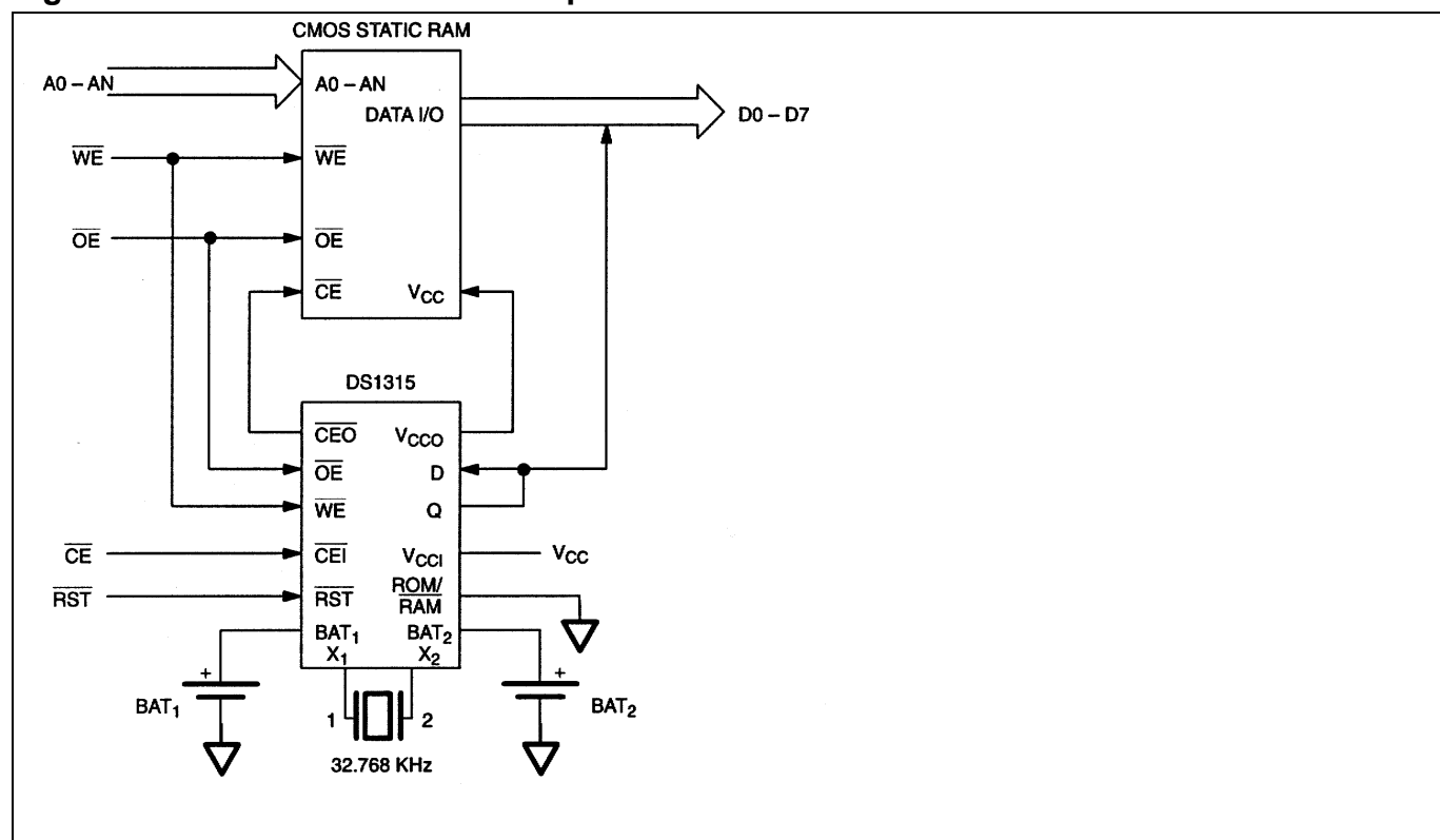
Figure 3. DS1315-to-RAM/Time Chip Interface
