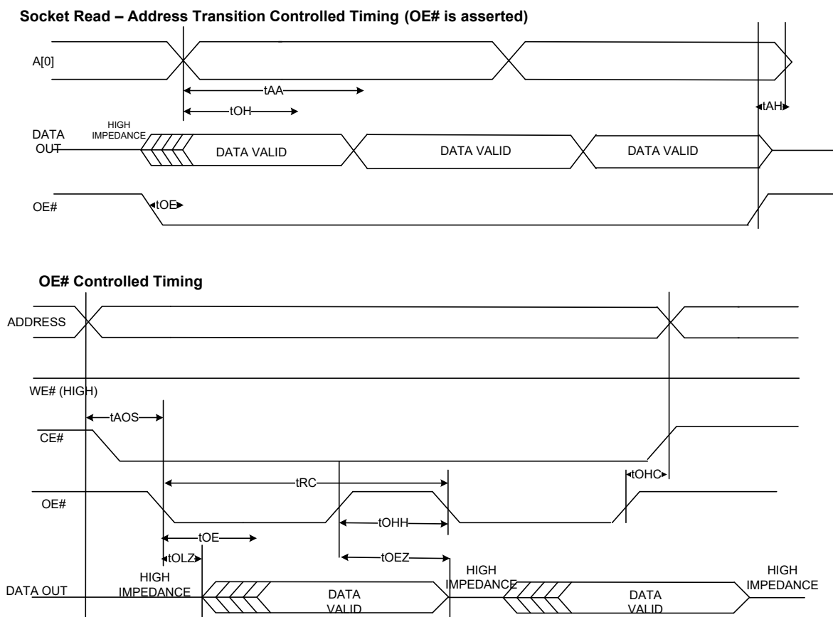
Figure 15. Non-multiplexed Asynchronous SRAM Read Timing
