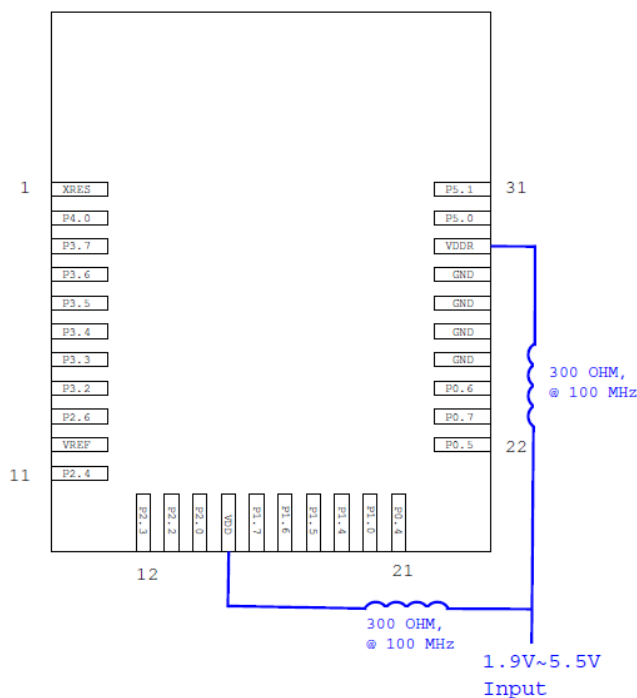
Figure 7. Recommended Host Schematic Options for a Single Supply Option
