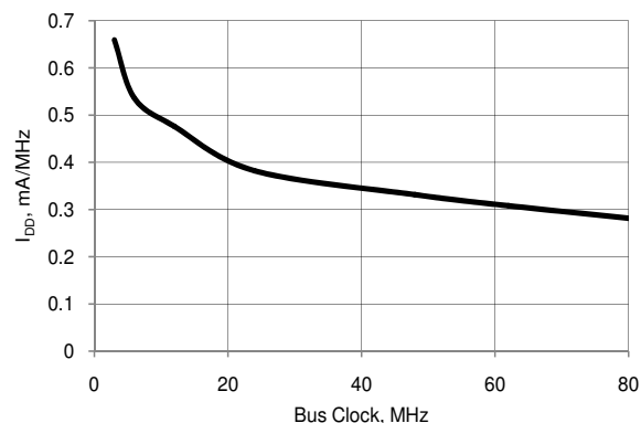
Figure 11-2. I_{DD} vs Frequency at 25^\circ\text{C}
