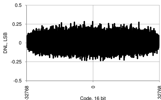
Figure 11-37. Delta-sigma ADC DNL vs Output Code, 16-bit, 48 ksps, 25 °C V DDA = 3.3 V
