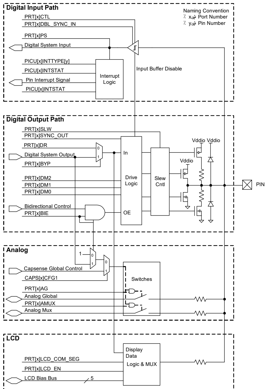
Figure 6-8. GPIO Block Diagram
