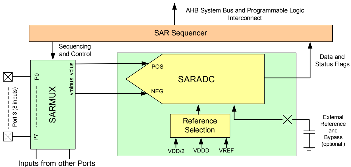
Figure 4. SAR ADC System Diagram
