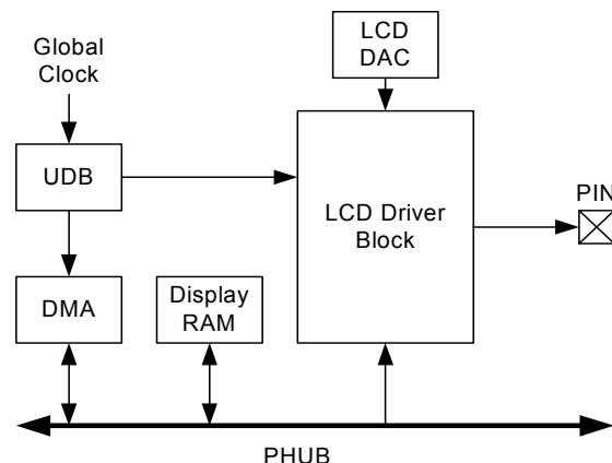
Figure 8-10. LCD System
