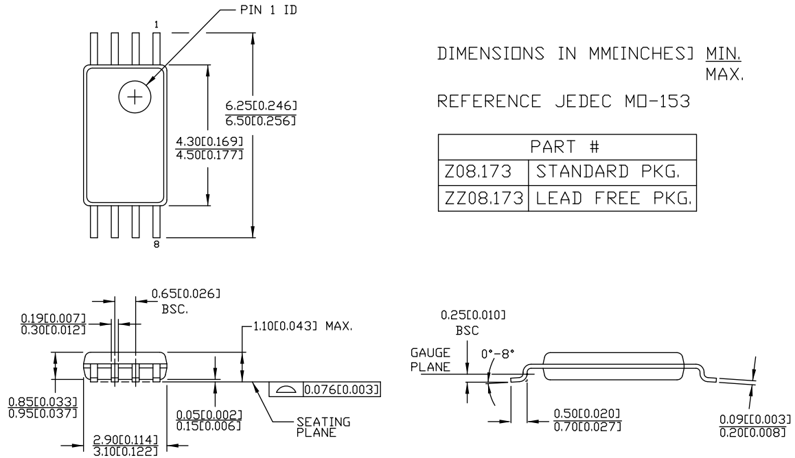
Figure 6. 8-pin TSSOP (4.40 mm Body) Z08.173/ZZ08.173 Package Outline, 51-85093
