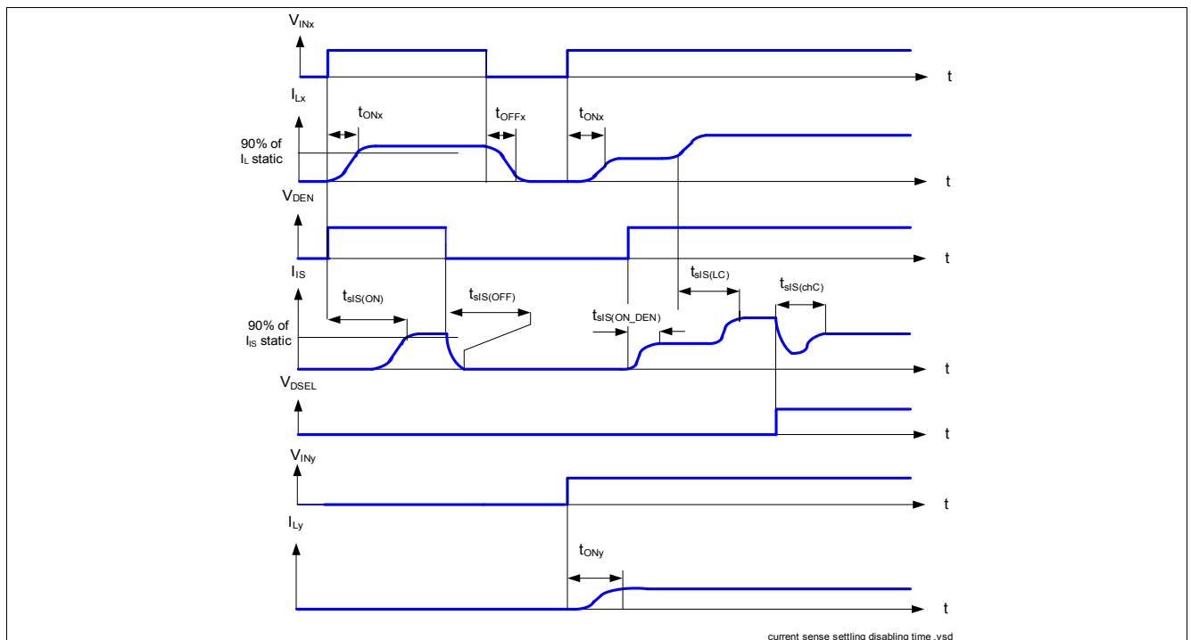
Figure 22 Current Sense Settling / Disabling Timing
