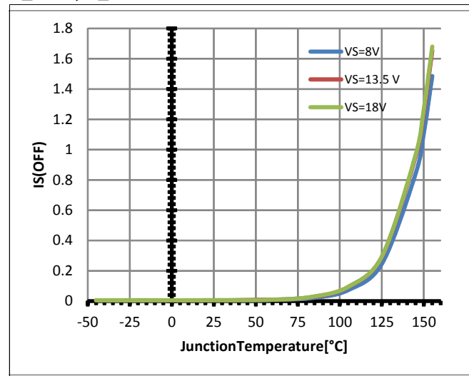
Standby Current for Whole Device with Load.
