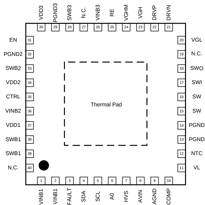
Figure 2. Pin Configuration
