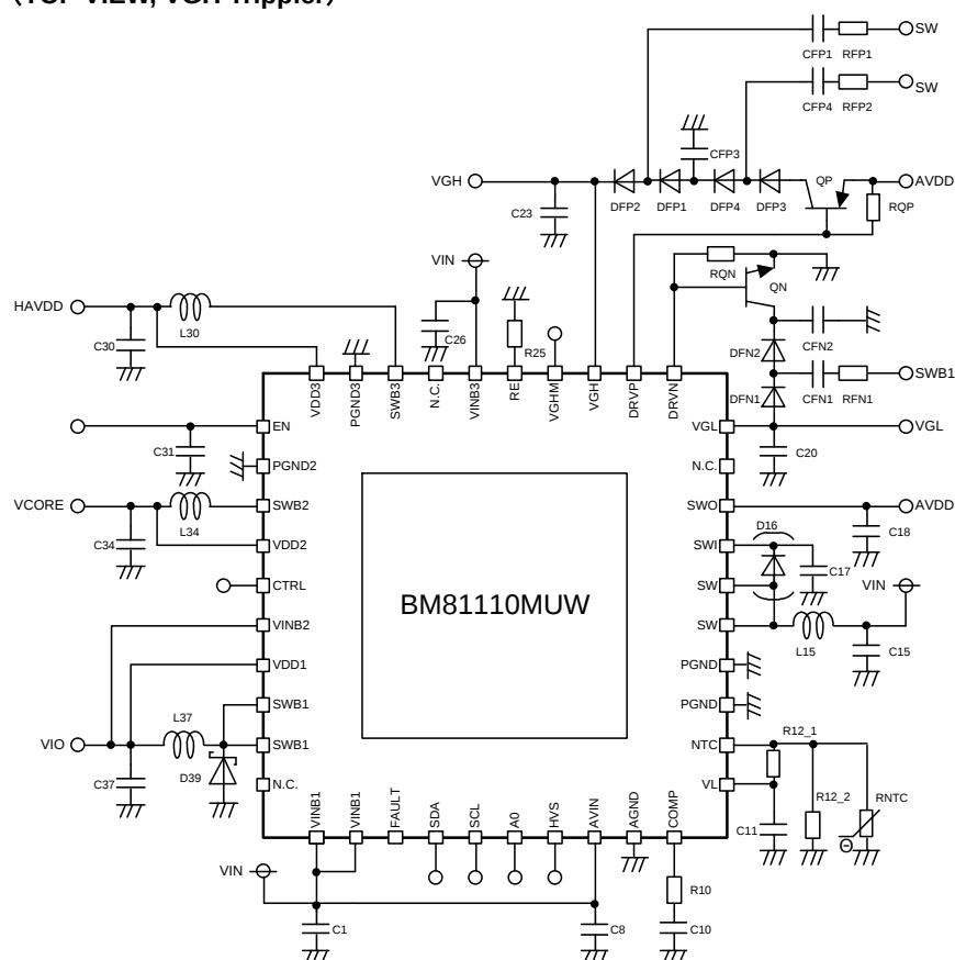
Figure 41. Example Application
