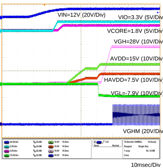
Figure 8. Power-on 2 (VGL driven AVDD switch node)
