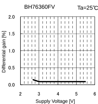
Fig.47 DG vs. Supply Voltage
