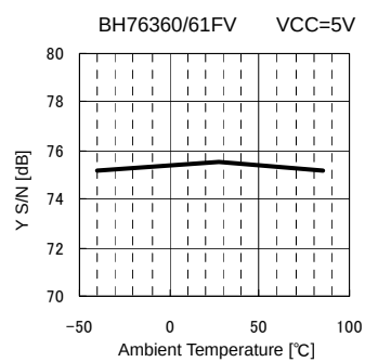
Fig.56 SN_{\gamma} vs. Ambient Temperature
