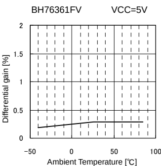
Fig.50 DG vs. Ambient Temperature
