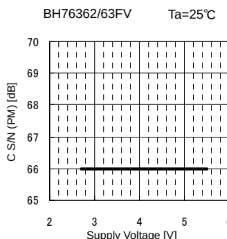
Fig.99 SN_{CP} vs. Supply Voltage
