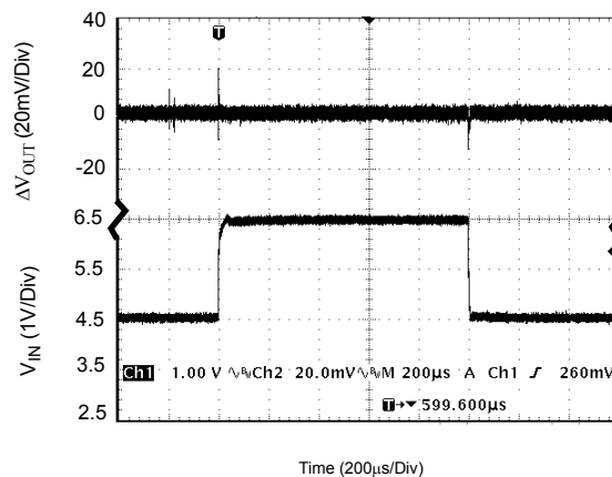
Figure 15. Line Transient Response (Conditions: V IN =4.5V to 6.5V, V OUT =2.5V, I OUT =200mA, C IN =1µF, C OUT =10µF)
