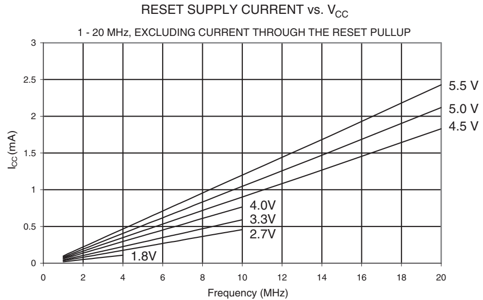
Figure 21-52. Reset Supply Current vs. V_{CC} (1 - 20 MHz, Excluding Current Through the Reset Pull-up)
