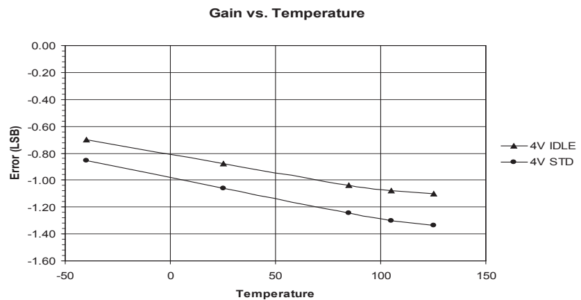
Figure 28-27. Analog to Digital Converter GAIN vs. V_{CC}
