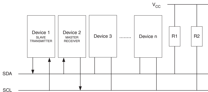
Figure 19-18. Data Transfer in Slave Transmitter Mode
