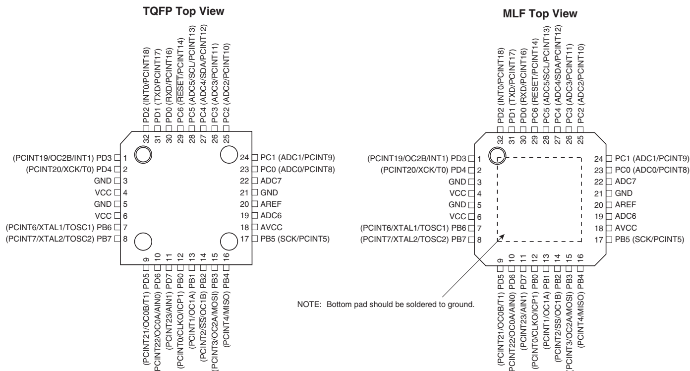
Figure 1-1. Pinout ATmega48/88/168
