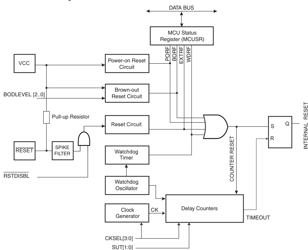
Figure 8-1. Reset Logic
