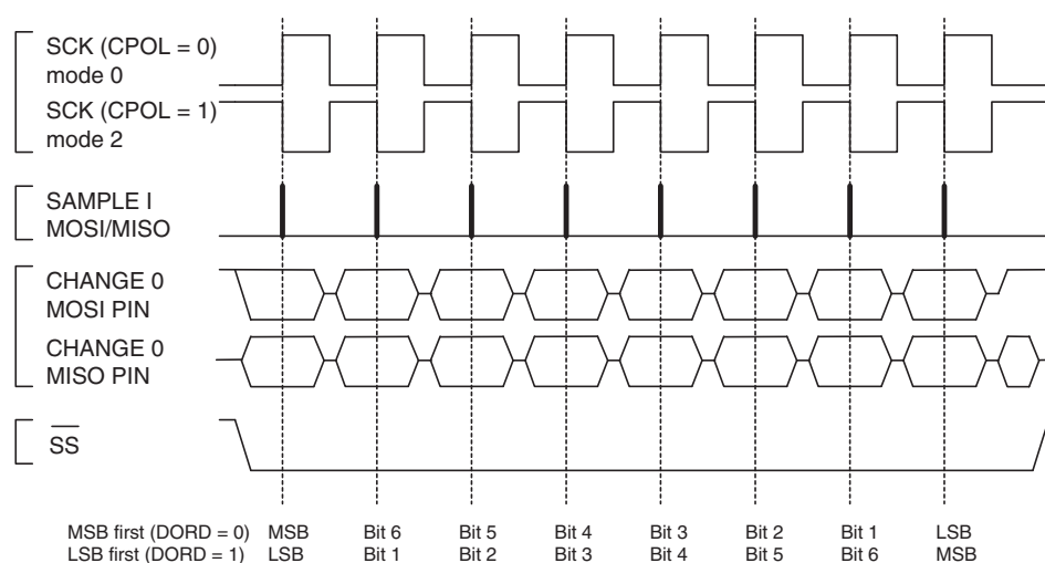
Figure 16-3. SPI Transfer Format with CPHA = 0
