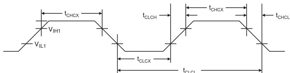
Figure 26-1. External Clock Drive Waveforms
